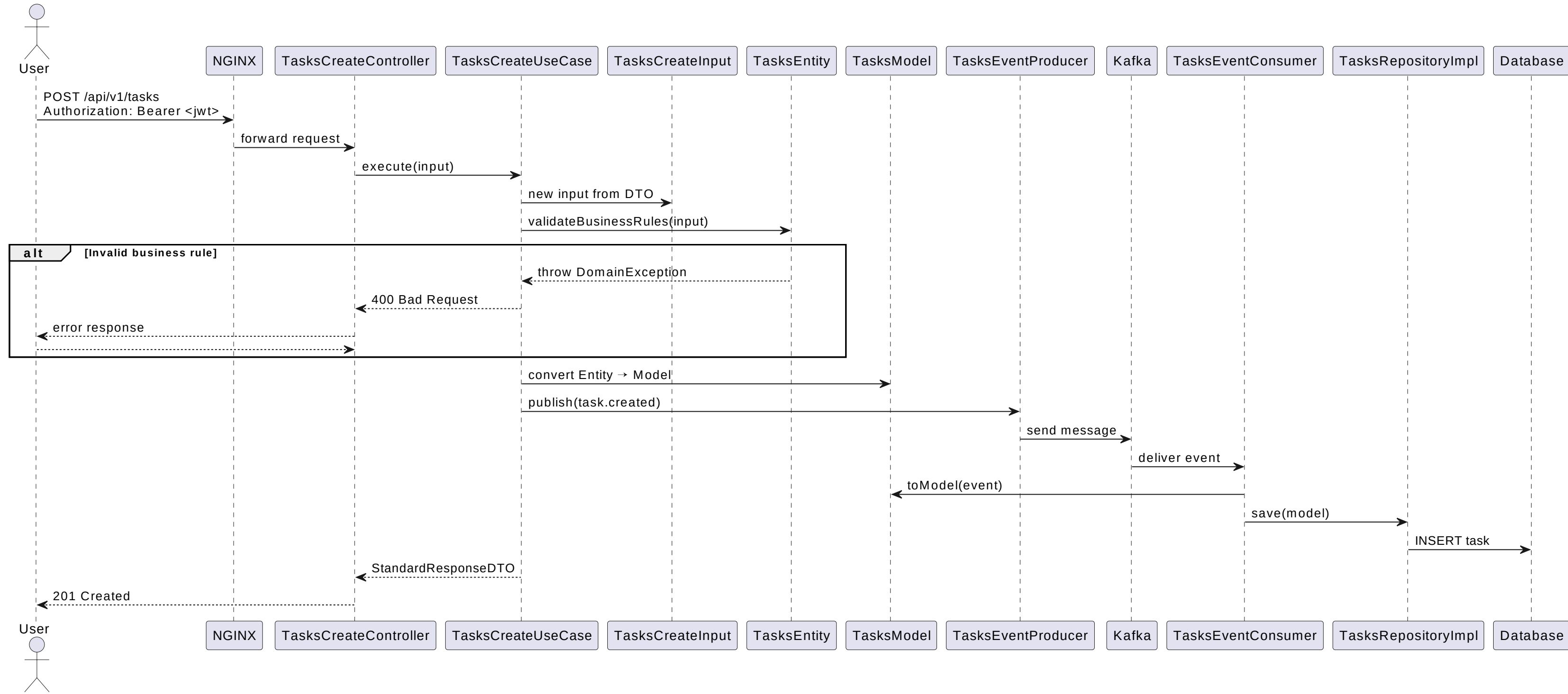
Sequence Diagram - POST /api/v1/tasks
